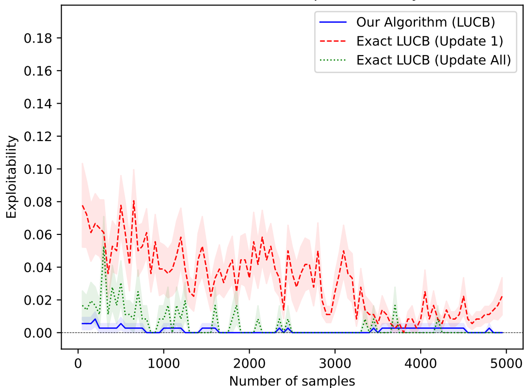
Kuhn Poker, Exact Computation, Player x
